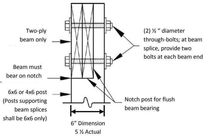
Notched Post
