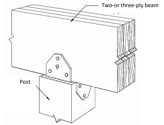
Post Cap
