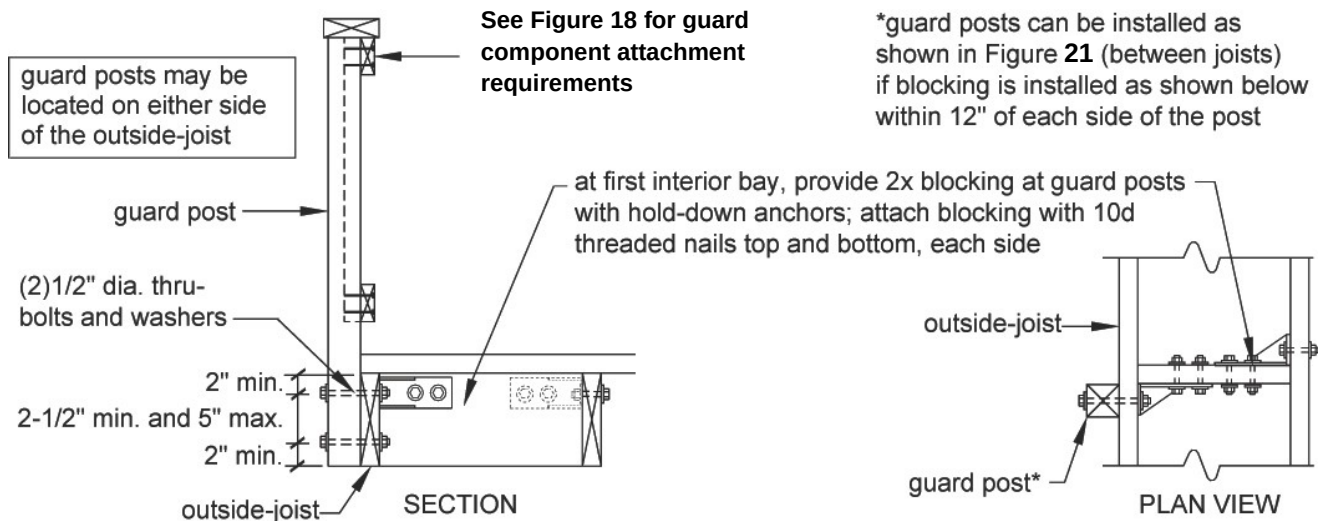
Figure 20. Guard Post to Outside Joist Example
