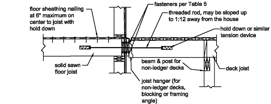
Figure 17. Lateral Load Device with Joists Parallel to Deck Joists
