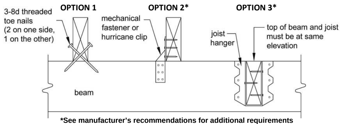
Figure 5. Joist-to-Beam Detail
