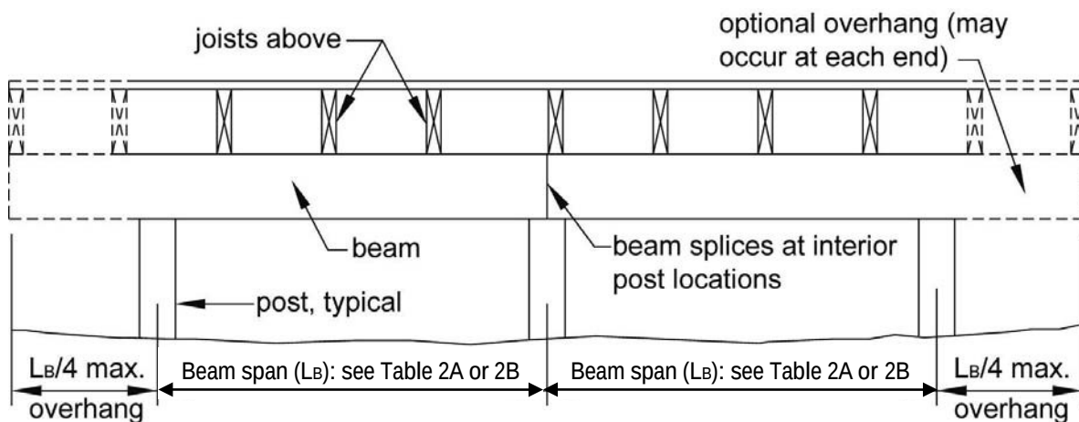
Figure 3. Beam Span
